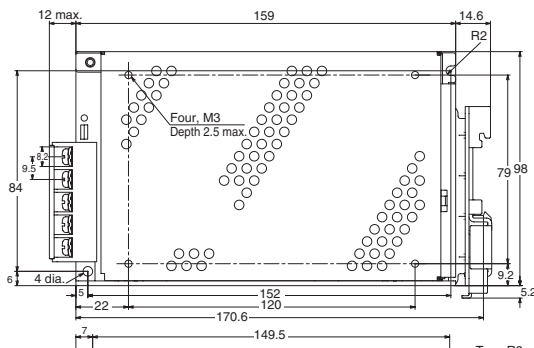
Panel mounting holes dimensions
