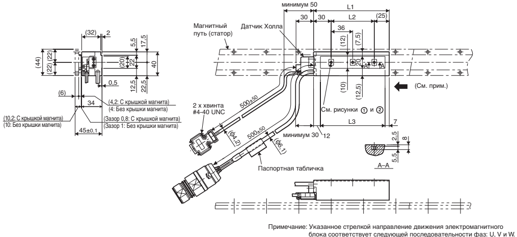
◎ SGLFW-20A090A□□
