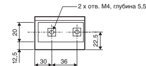
◎ SGLFW-20A090A□□
