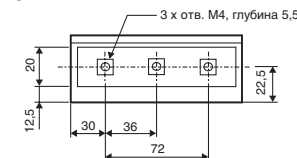
◎ SGLFW-20A120A□□
